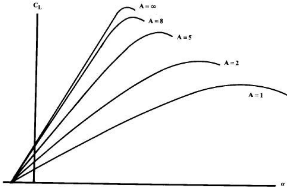
Figure 2. Effect of aspect ratio on lift
