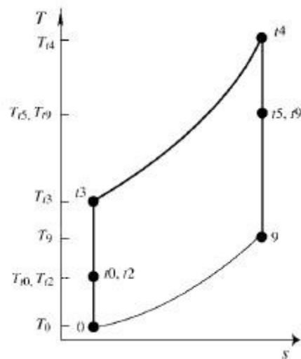
Figure 4. T-s diagram for an ideal turbojet
