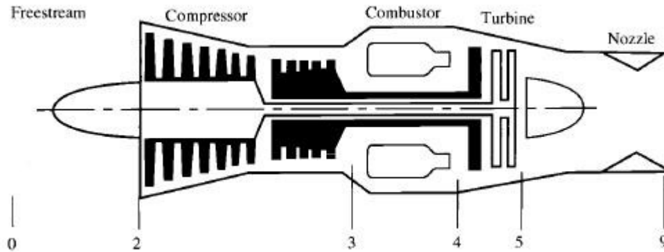
Figure 3. Station numbering for an ideal turbojet
