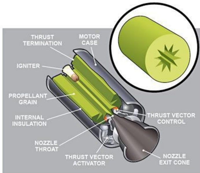
Figure 6. Cut away picture of a solid rocket and its components
