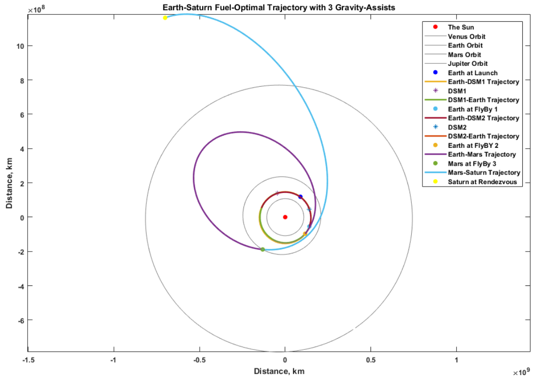
Figure 6.4: An Earth-Saturn Optimal Trajectory with 3 Gravity-Assist Maneuvers
