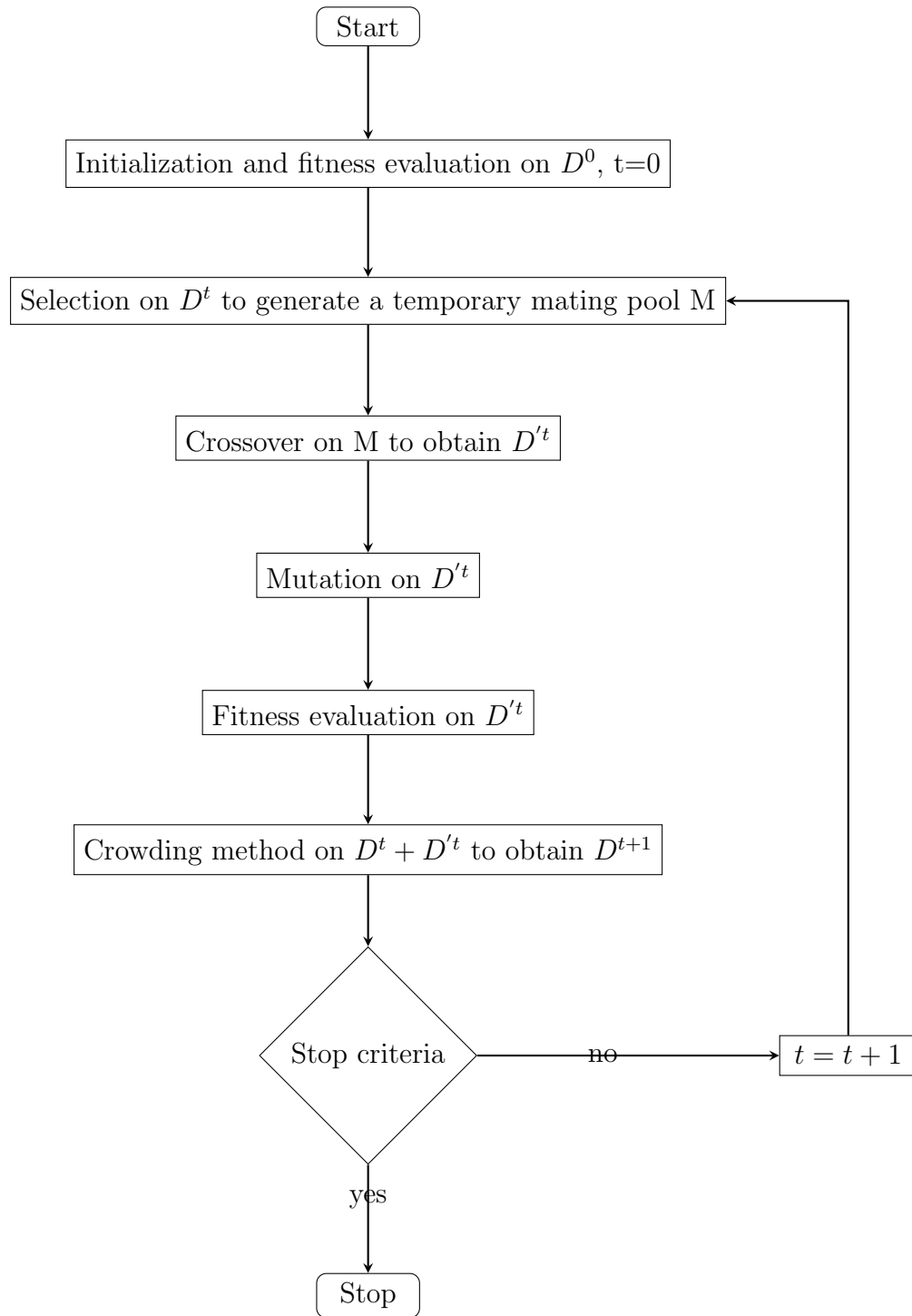
Figure 4.4: TCGA Flow Chart [3]
