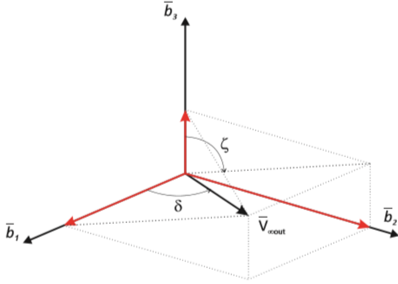
Figure 3.1: Gravity-Assist Orientation [2].
