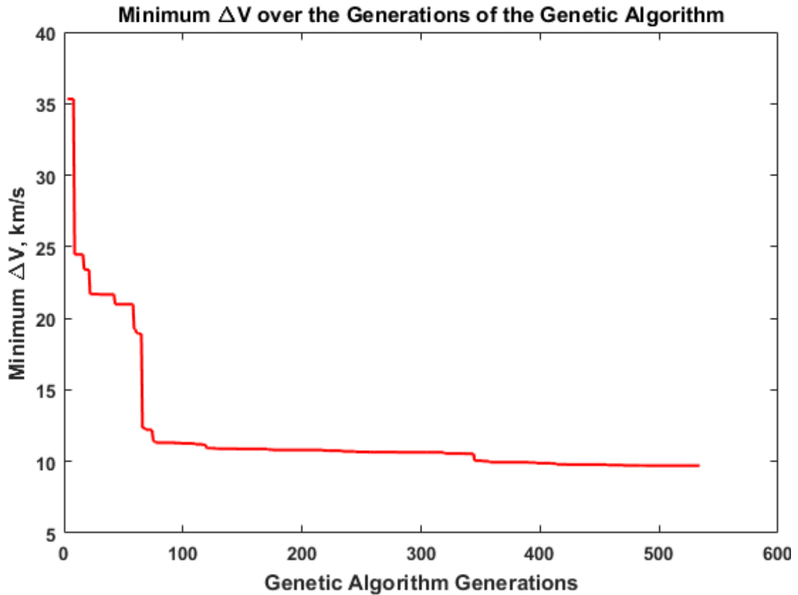
Figure 6.3: The Minimum \Delta V over the Generations of the Genetic Algorithm for 4 Gravity-Assists
