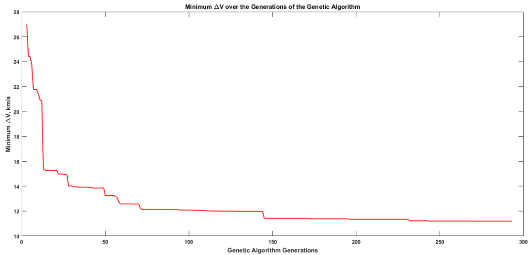
Figure 6.6: The Minimum \Delta V over the Generations of the Genetic Algorithm for 3 Gravity-Assists
