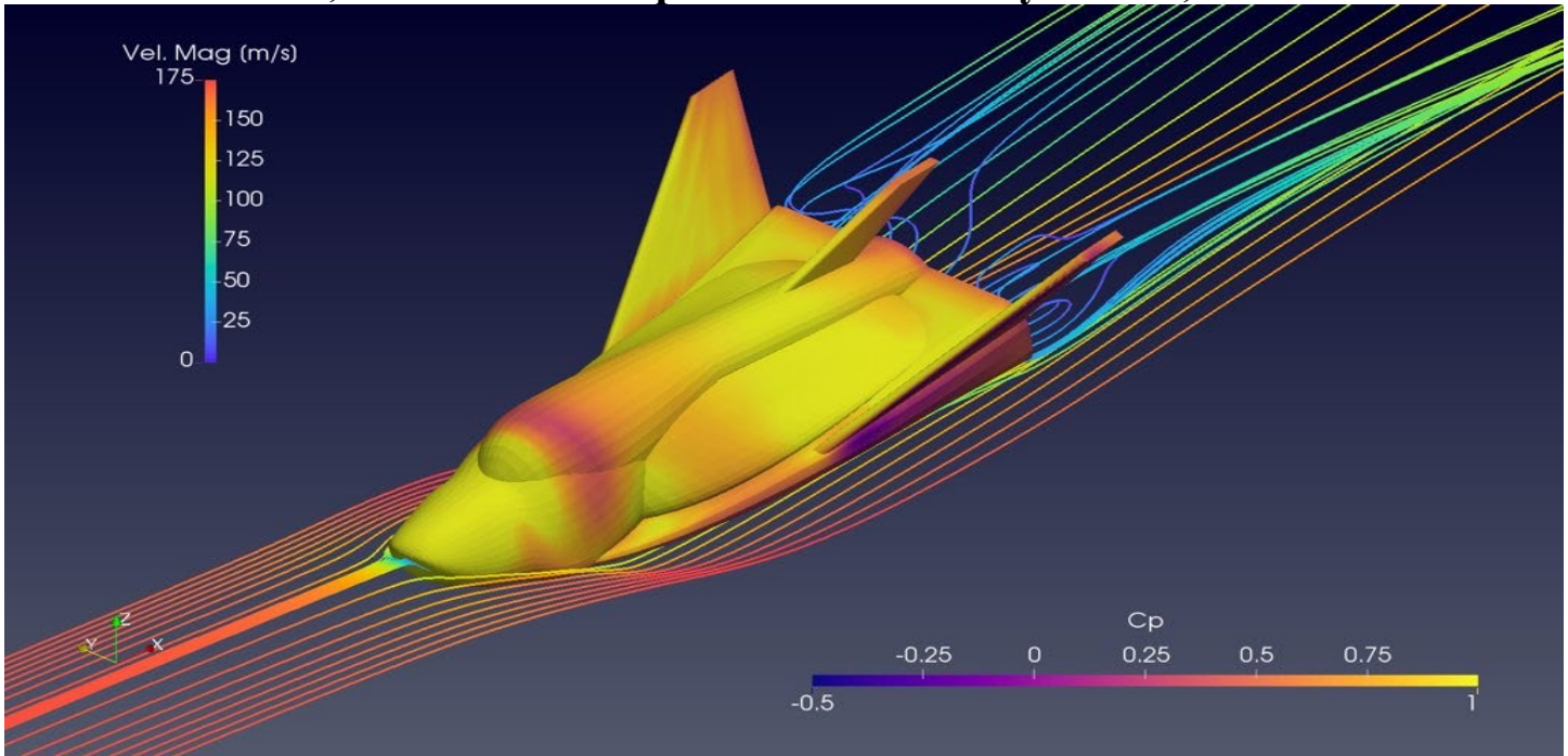
(Figure-RANS Simulation of the NASA HL-20 Spaceplane at Re-entry Config., Courtesy of NASA)
