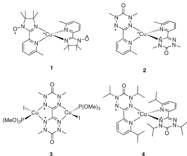
Chart 1. Copper(I) Radical Complexes 1–4
