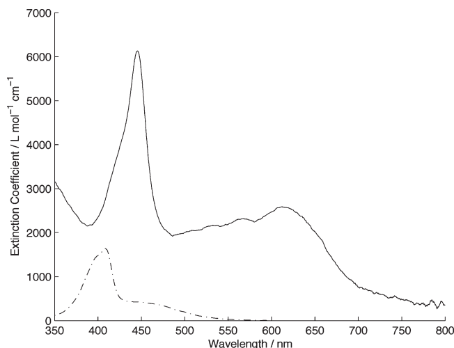
Figure 2. Electronic absorption spectrum of 4 in dichloromethane (solid line). The electronic absorption of 1,5-diisopropyl-3-(2'-pyridyl)verbazyl (broken line) is shown for comparison.
