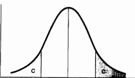
FIGURE A.2 AREA BEYOND Z
