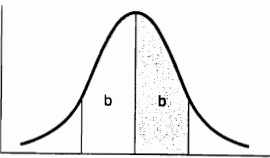
FIGURE A.1 AREA BETWEEN MEAN AND Z
