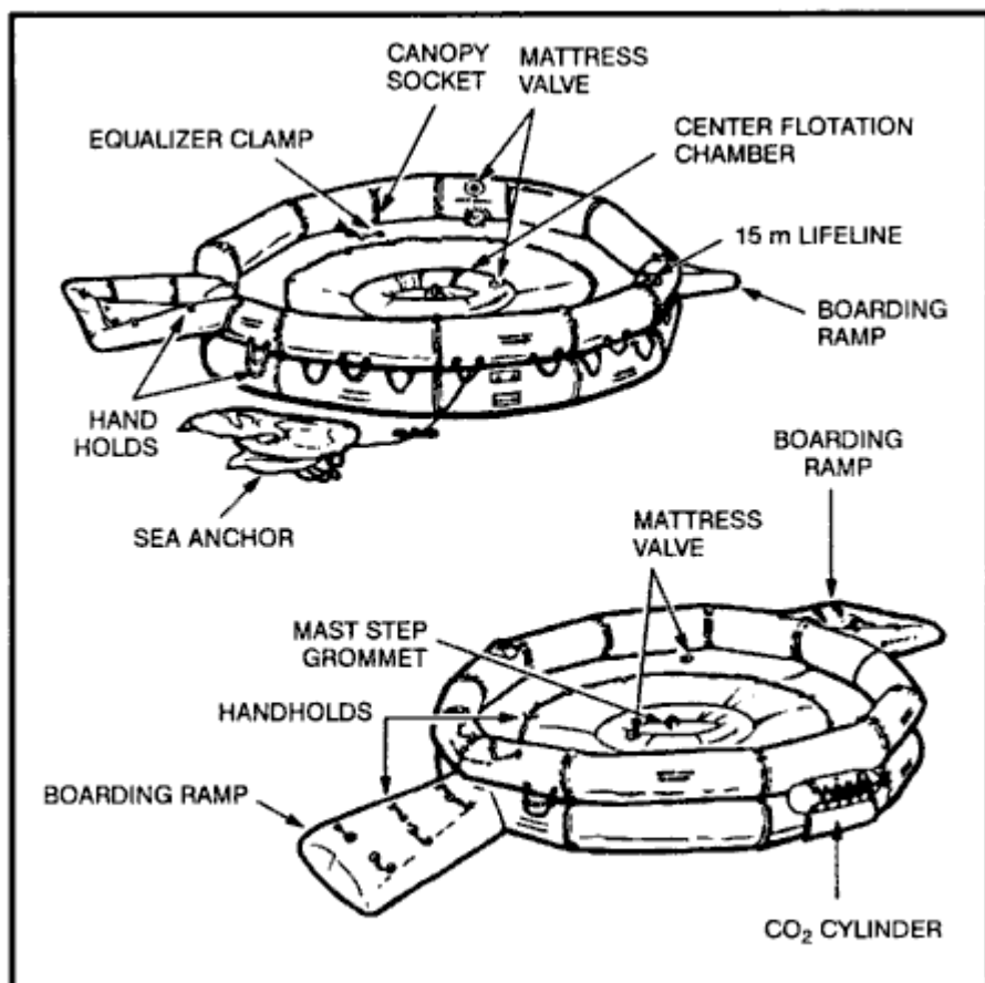
Figure 16-15. Twenty-man raft.
